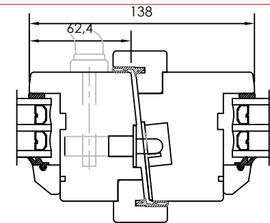
HORIZONTAL CS OPTION - Two horizontal abutting sashes.
