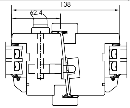
HORIZONTAL CS OPTION - Two horizontal abutting sashes.
