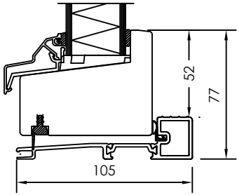
VERTICAL CS OPTION - Low handicap threshold.
